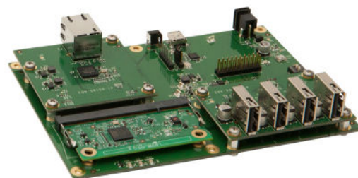
Remote Extender Evaluation Board with GMII, USB Hub and Core Modules
