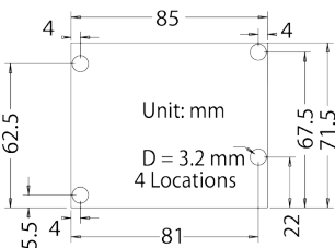
Local and Remote Extender Dimensions
