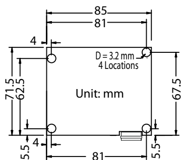
Local/Remote Extender Dimensions
