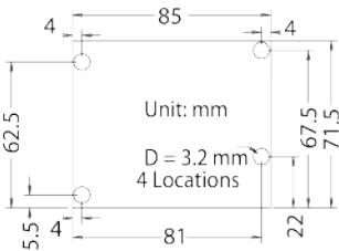
Local and Remote Extender Dimensions
