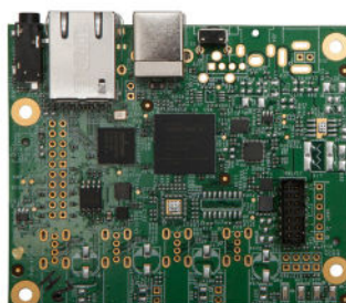
Local Extender
